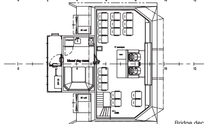
Bridge deck
