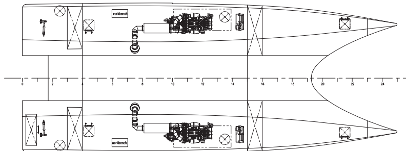
Below maindeck
